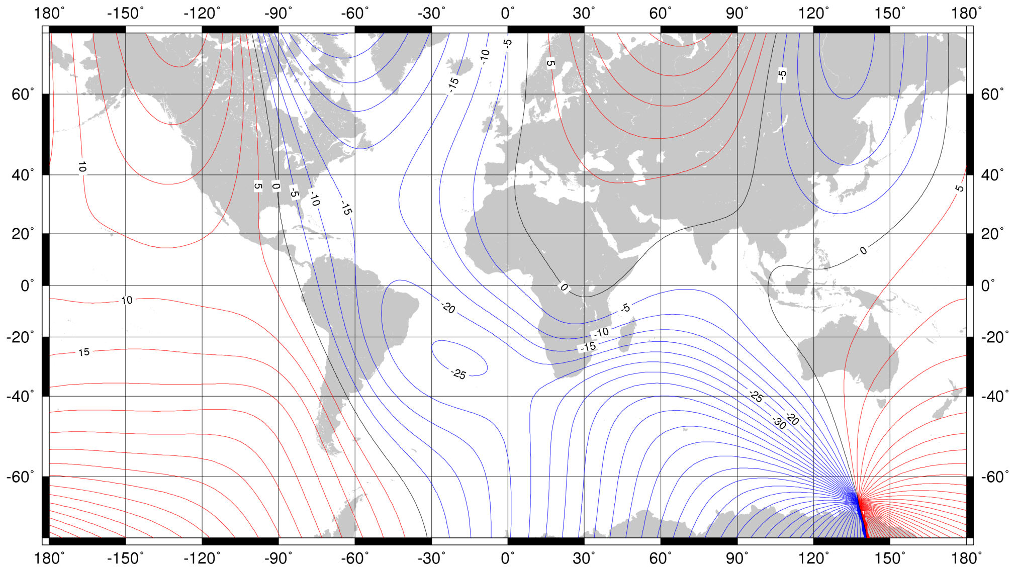
Declination (magnetic variation) at 2010.0 from the World Magnetic Model (WMM2010). Red - positive (east), blue - negative (west), black - zero (agonic line). Contour interval is 5° and projection is Mercator. This is an example of an isogonic chart. Credit: British Geological Survey (Natural Environment Research Council).
