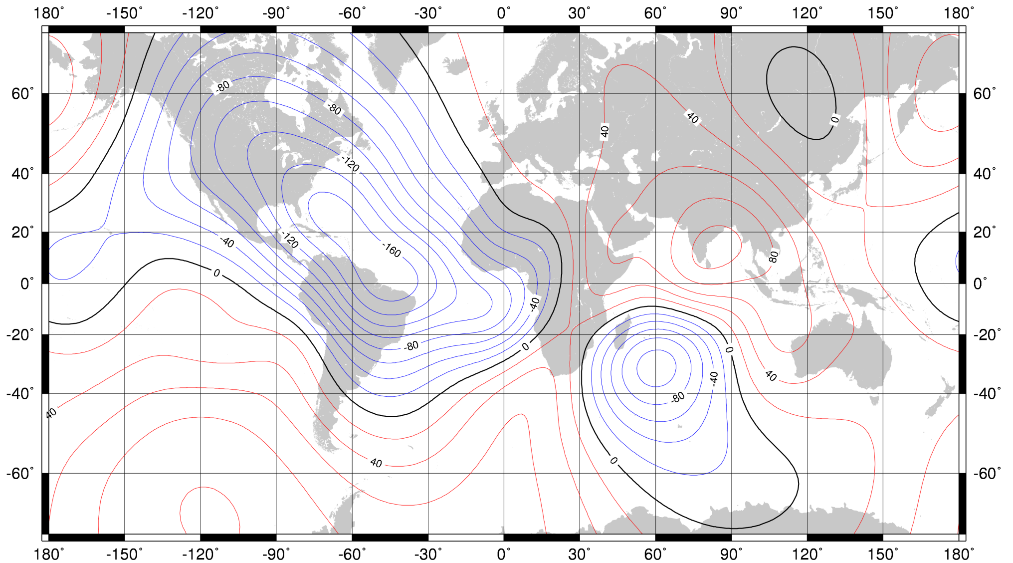
Annual rate of change of vertical intensity for 2010.0 to 2015.0 from the World Magnetic Model (WMM2010). Red - positive change (down), blue - negative change (up), black - zero change. Contour interval is 20 nT/year and projection is Mercator. This is an example of an isoporic chart. Credit: British Geological Survey (Natural Environment Research Council).
