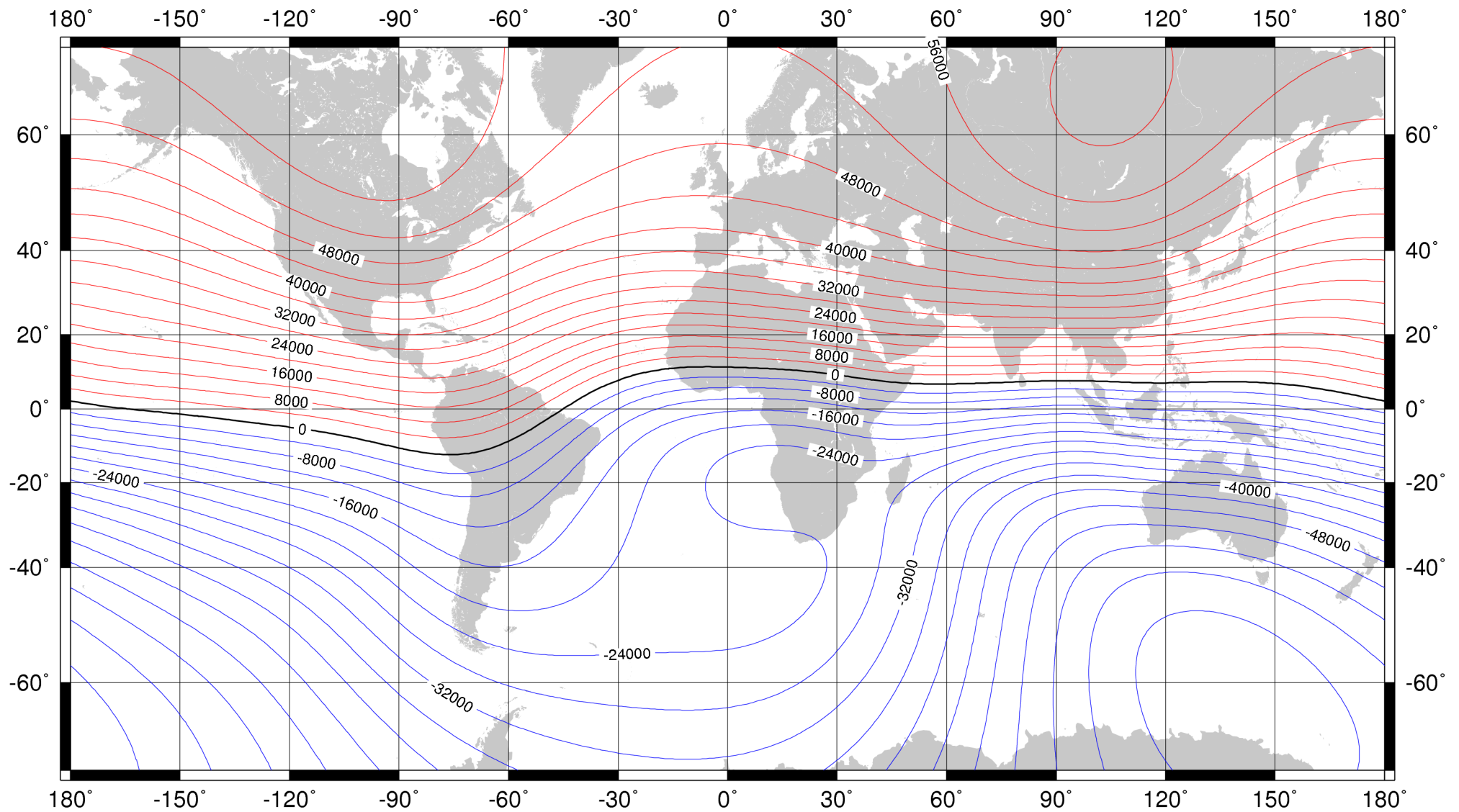
Vertical intensity (Z) at 2010.0 from the World Magnetic Model (WMM2010). Red - positive (down), blue - negative (up), black - zero. Contour interval is 4000 nT and projection is Mercator. This is an example of an isodynamic chart. Credit: British Geological Survey (Natural Environment Research Council).
