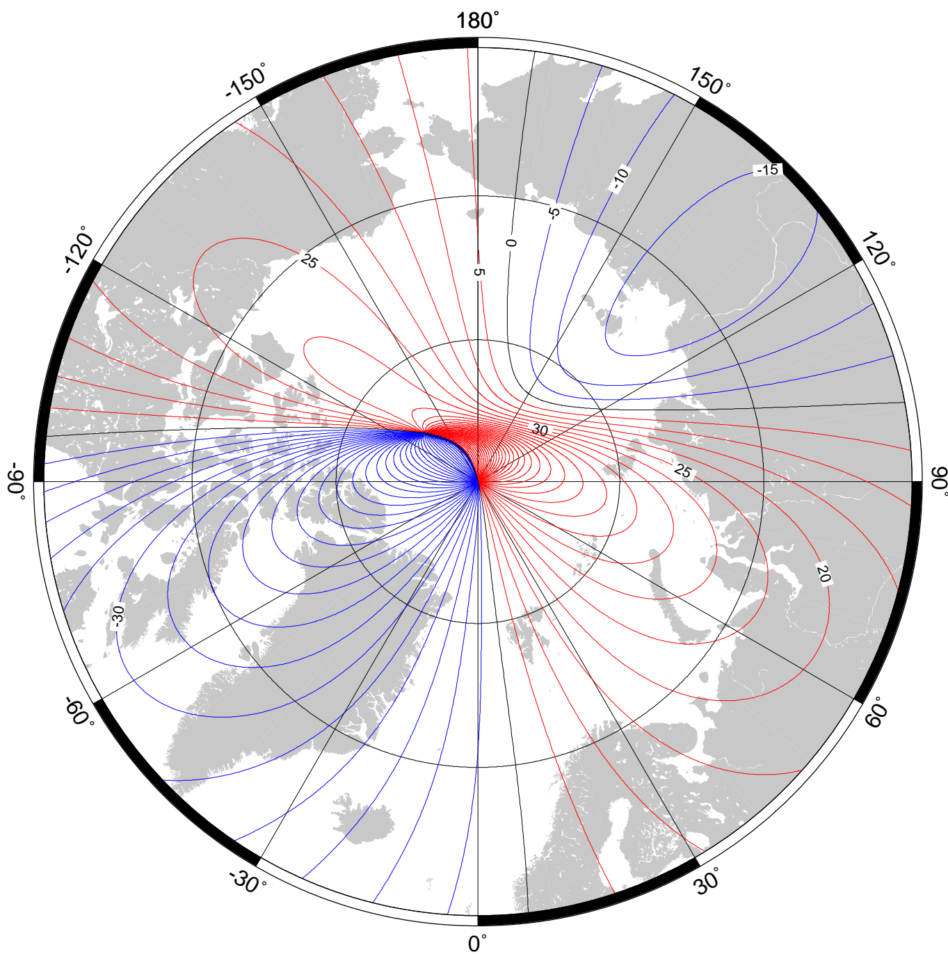
Declination (magnetic variation) in region of north pole at 2010.0 from the World Magnetic Model (WMM2010). Red - positive (east), blue - negative (west), black - zero. Contour interval is 5° and projection is Polar Stereographic. Credit: British Geological Survey (Natural Environment Research Council).
