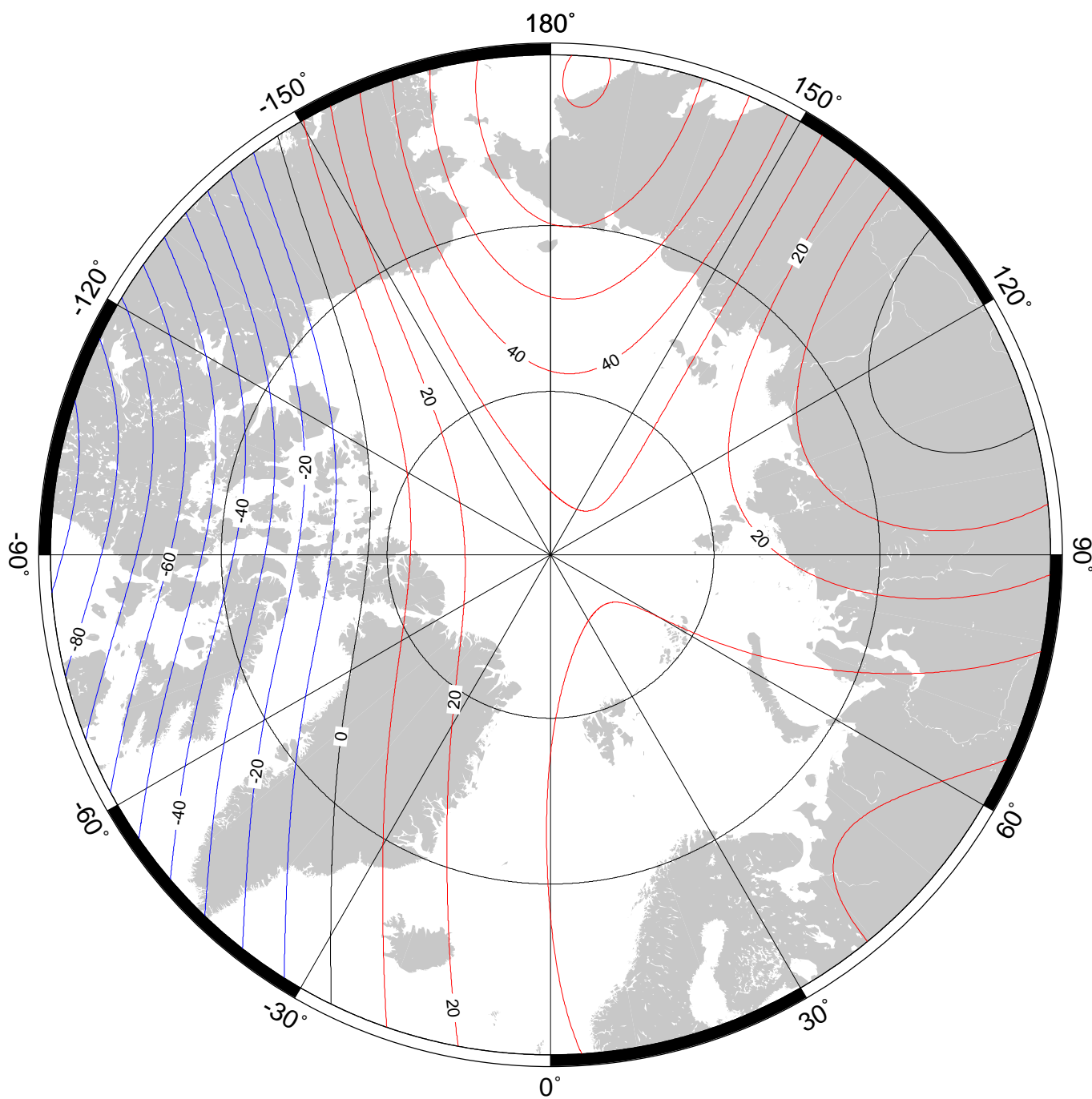
Annual rate of change of vertical component in region of north pole for 2010.0 to 2015.0 from the World Magnetic Model (WMM2010). Red - positive change, blue - negative change, black - zero change. Contour interval is 10 nT/year and projection is Polar Stereographic. Credit: British Geological Survey (Natural Environment Research Council).
