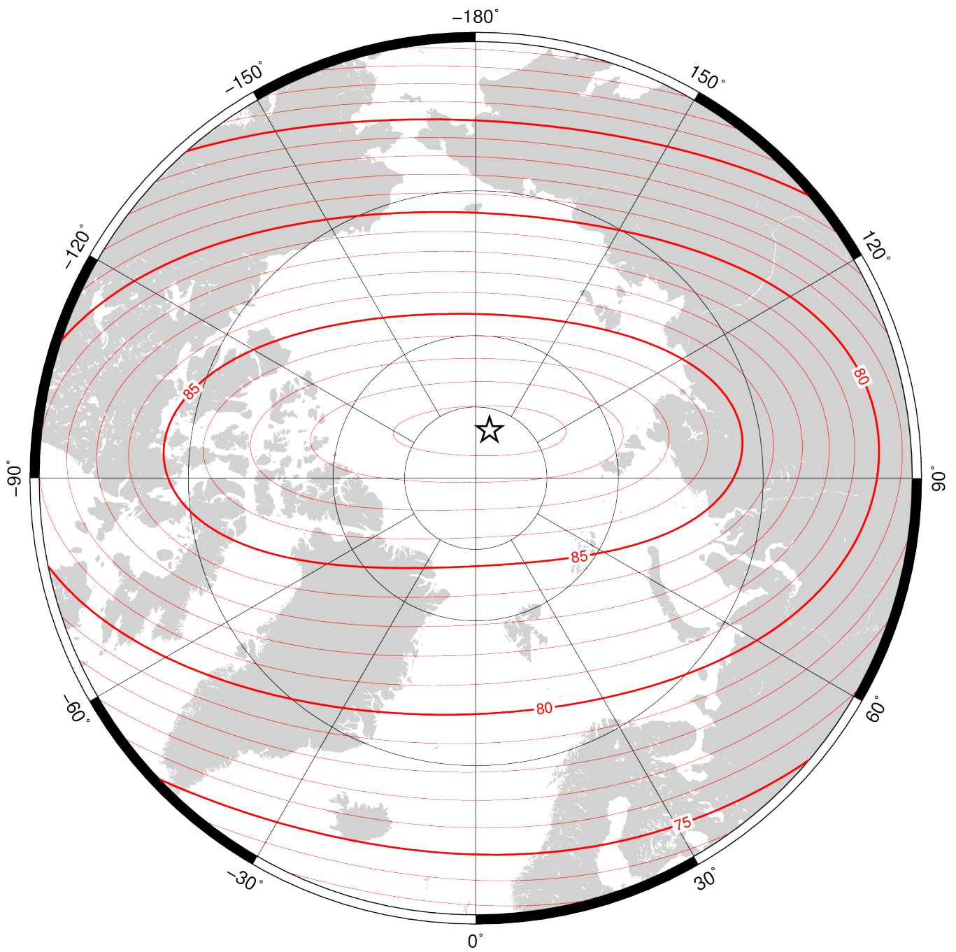
Inclination (magnetic dip) in region of north pole at 2020.0 from the World Magnetic Model (WMM2020). Contour interval is 1^\circ , white star is location of a magnetic pole and projection is Polar Stereographic. Credit: British Geological Survey (UK Research and Innovation).
