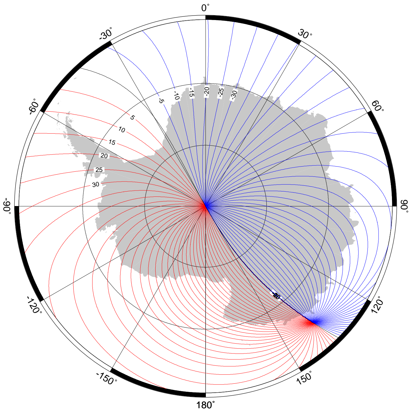
Declination (magnetic variation) in region of south pole at 2010.0 from the World Magnetic Model (WMM2010). Red - positive (east), blue - negative (west), black - zero. Contour interval is 5° and projection is Polar Stereographic. Credit: British Geological Survey (Natural Environment Research Council).
