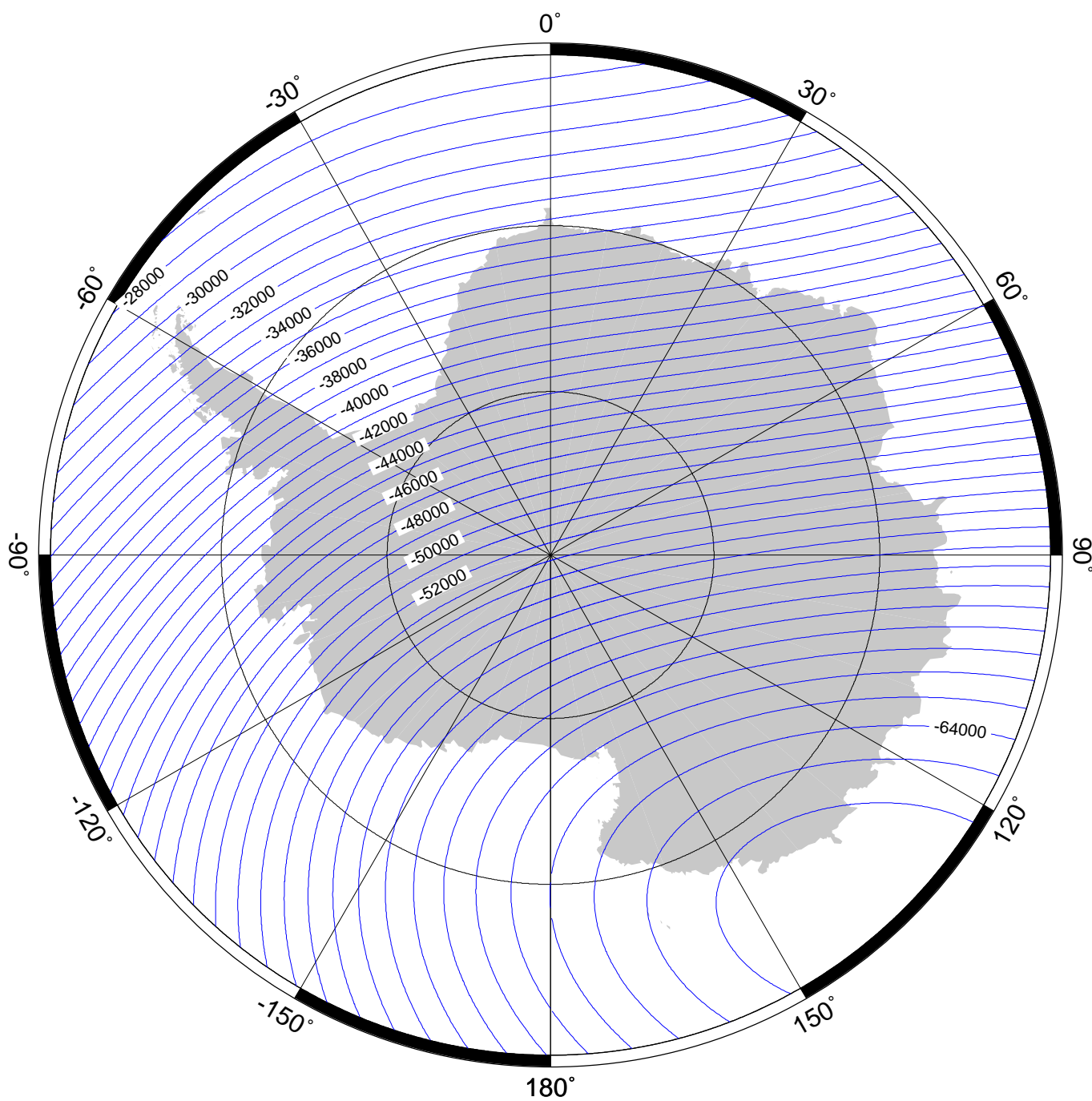
Vertical component (Z) in region of south pole at 2010.0 from the World Magnetic Model (WMM2010). Contour interval is 1000 nT and projection is Polar Stereographic. Credit: British Geological Survey (Natural Environment Research Council).
