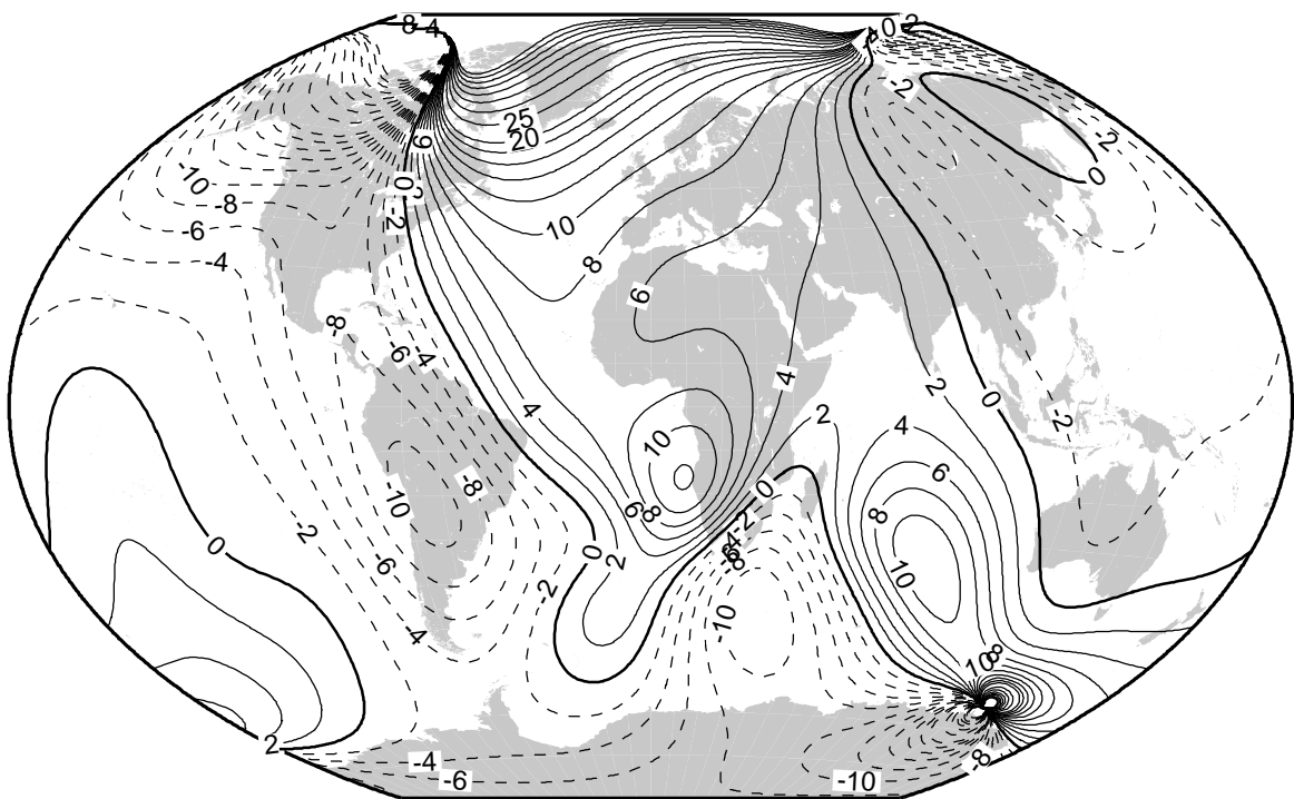
Secular variation of declination (min/yr) for 2010.0-2015.0
