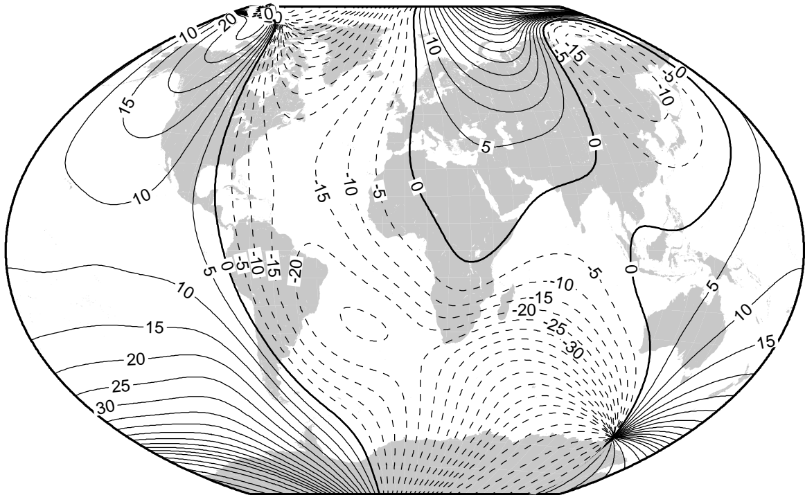
Declination (degrees) at 2010.0
