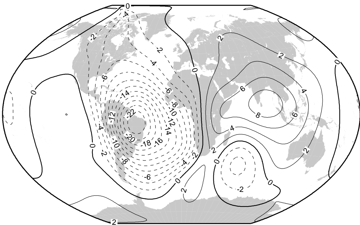
Secular variation of inclination (min/yr) for 2010.0-2015.0
