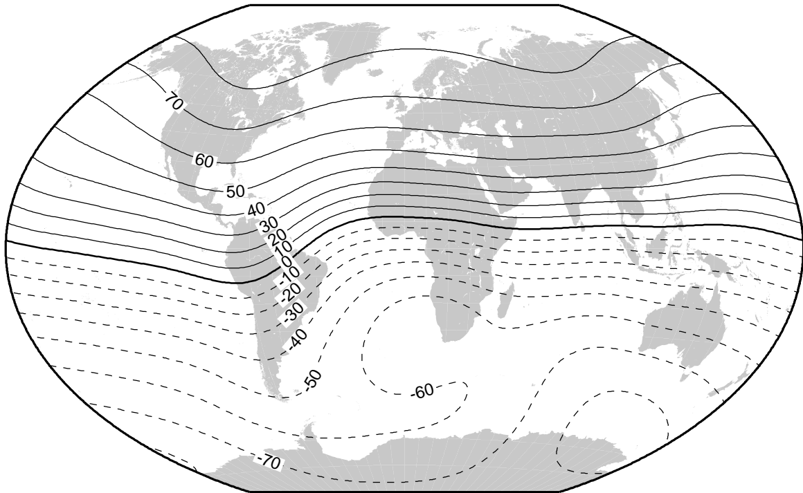
Inclination (degrees) at 2010.0
