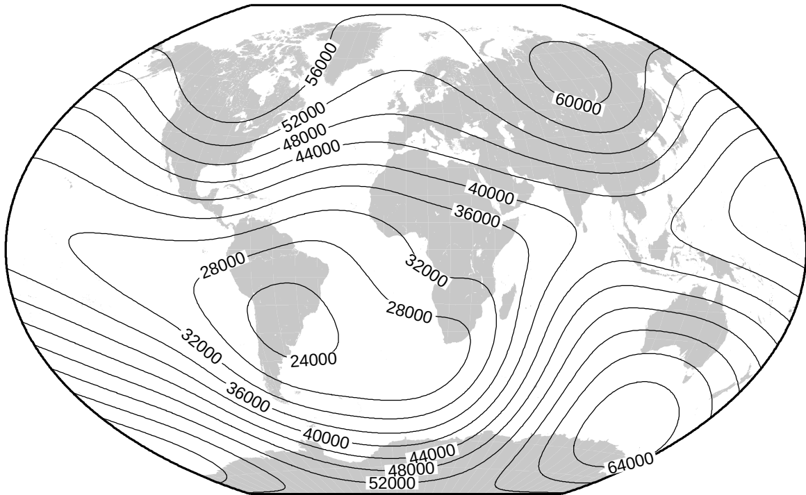
Total intensity (nT) at 2010.0
