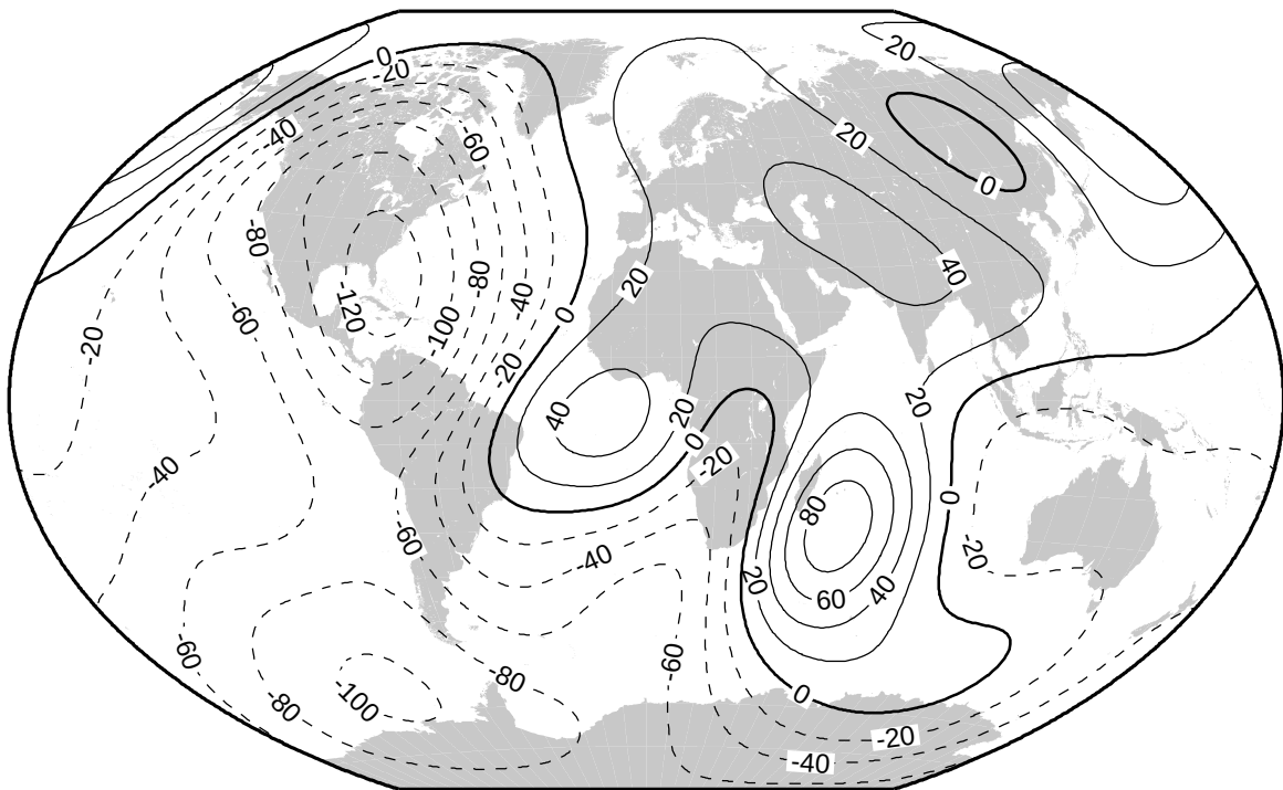
Secular variation of total intensity (nT/yr) for 2010.0-2015.0
