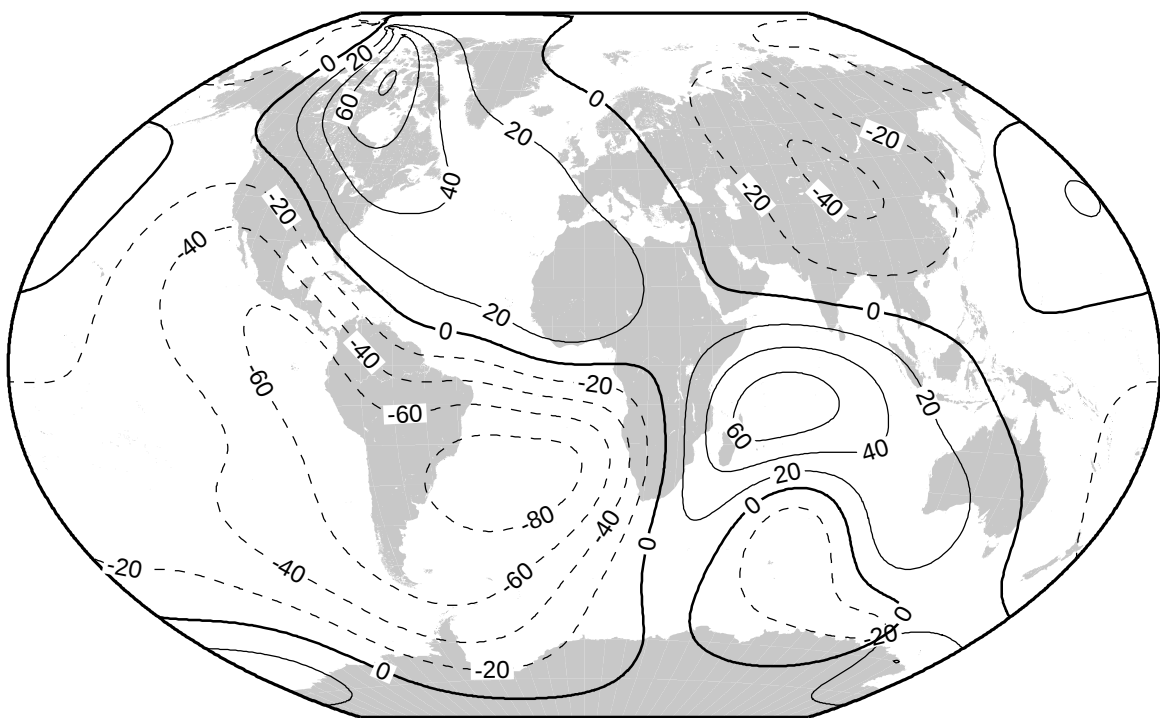
Secular variation of horizontal intensity (nT/yr) for 2010.0-2015.0
