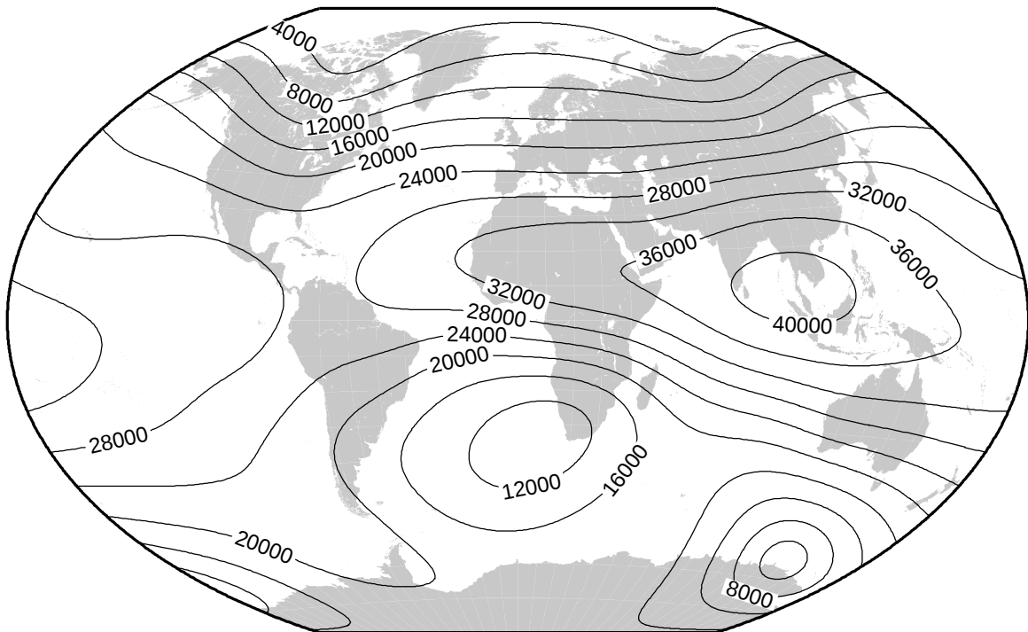
Horizontal intensity (nT) at 2010.0
