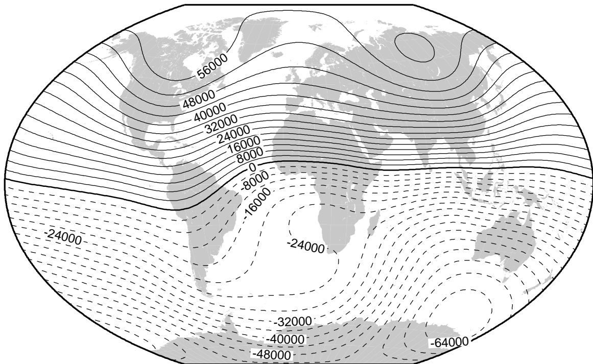
Vertical component (nT) at 2010.0
