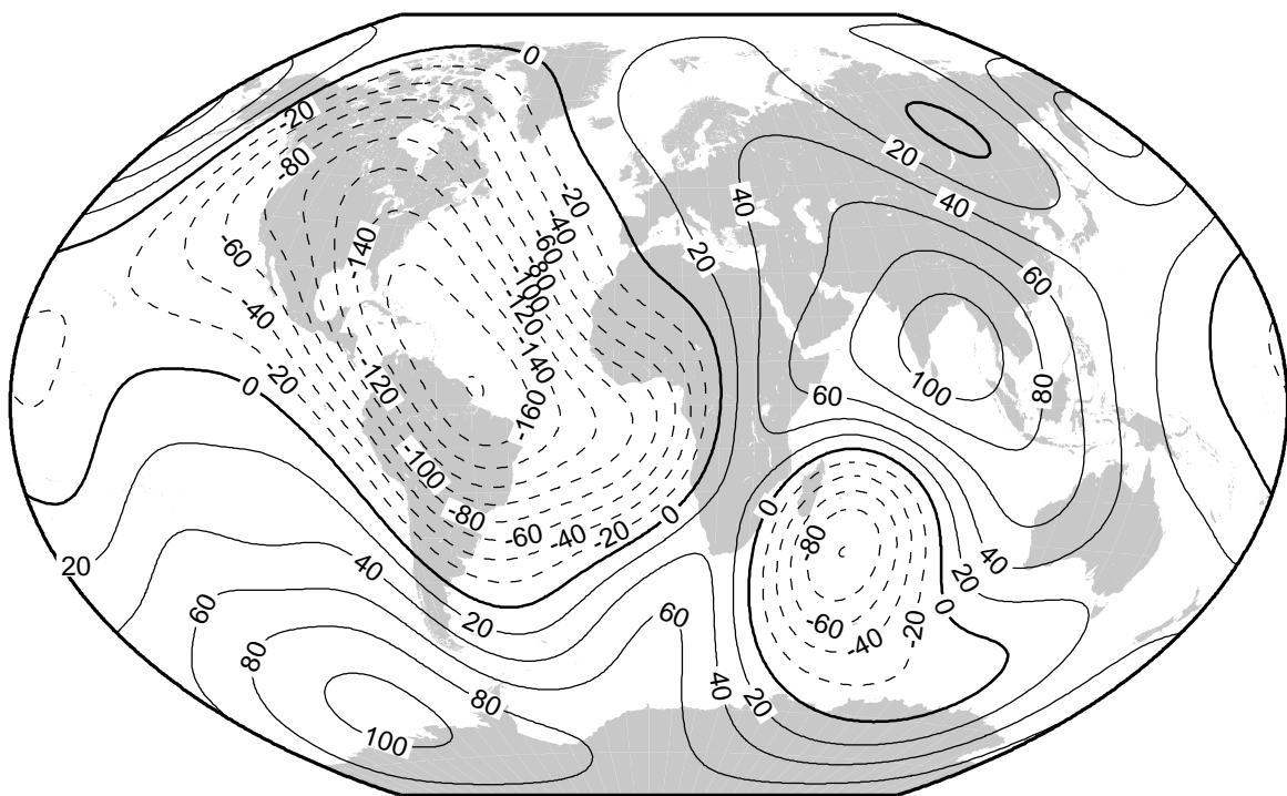
Secular variation of vertical component (nT/yr) for 2010.0-2015.0
